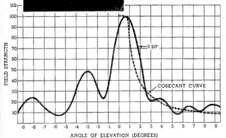
Radiation pattern of Model WA-25-XX with null fill-in and beam tilt of 0.65^\circ .
